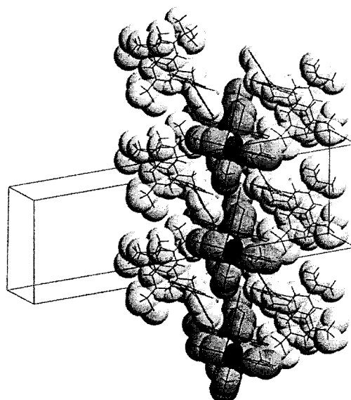
Figure 9. X-ray crystallographic structure of \text{Cy}_{3,5t\text{-Bz}}^+ , 2\text{MeSpB}^- showing vertical stacks of the subunit producing ladder-like structure with the borate (bold) and cyanine (light). (Reprinted with permission from ref 158. Copyright 1998 American Chemical Society.)
