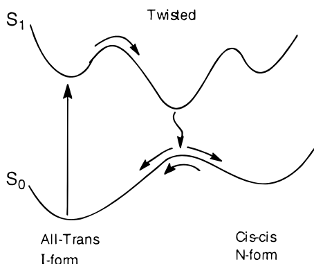
Figure 11. Schematic potential energy diagram for DOD-Cl ( 87 ) photolysis. (Reprinted with permission from ref 201. Copyright 1991 American Chemical Society.)
