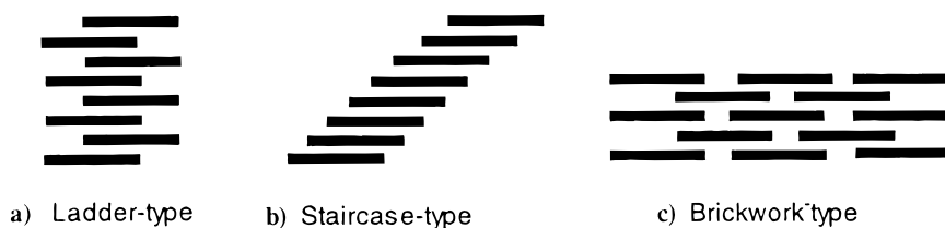
Figure 2. Schematic representation of the different arrangement of cyanine dyes in the solid surface and in solution. (Reprinted with permission from ref 61. Copyright 1996 American Chemical Society.)
