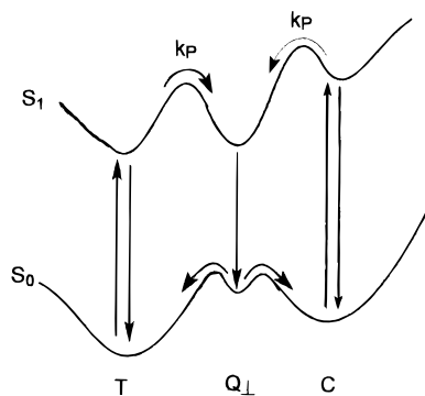
Figure 10. Potential energy diagram which explains the possible coexistence of the three isomers of 86 in organic solvent and in surfactant solution. The quinoid form is the intermediate structure between the cis and trans isomers.
