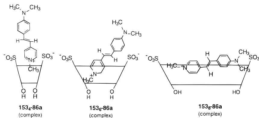
Figure 17. Estimated structures for 153 4 , 153 6 , and 153 8 complexes with 86a . (Reprinted with permission from ref 375. Copyright 1997 The Bulletin Chemical Society Japan.)
