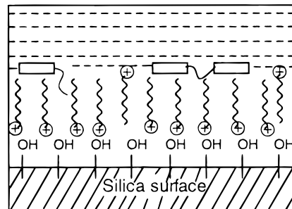
Figure 7. Schematic diagram of the orientation of monochromophoric ( 49 ) and bischromophoric dyes ( 50 ) on a CTAB-treated silica surface.
