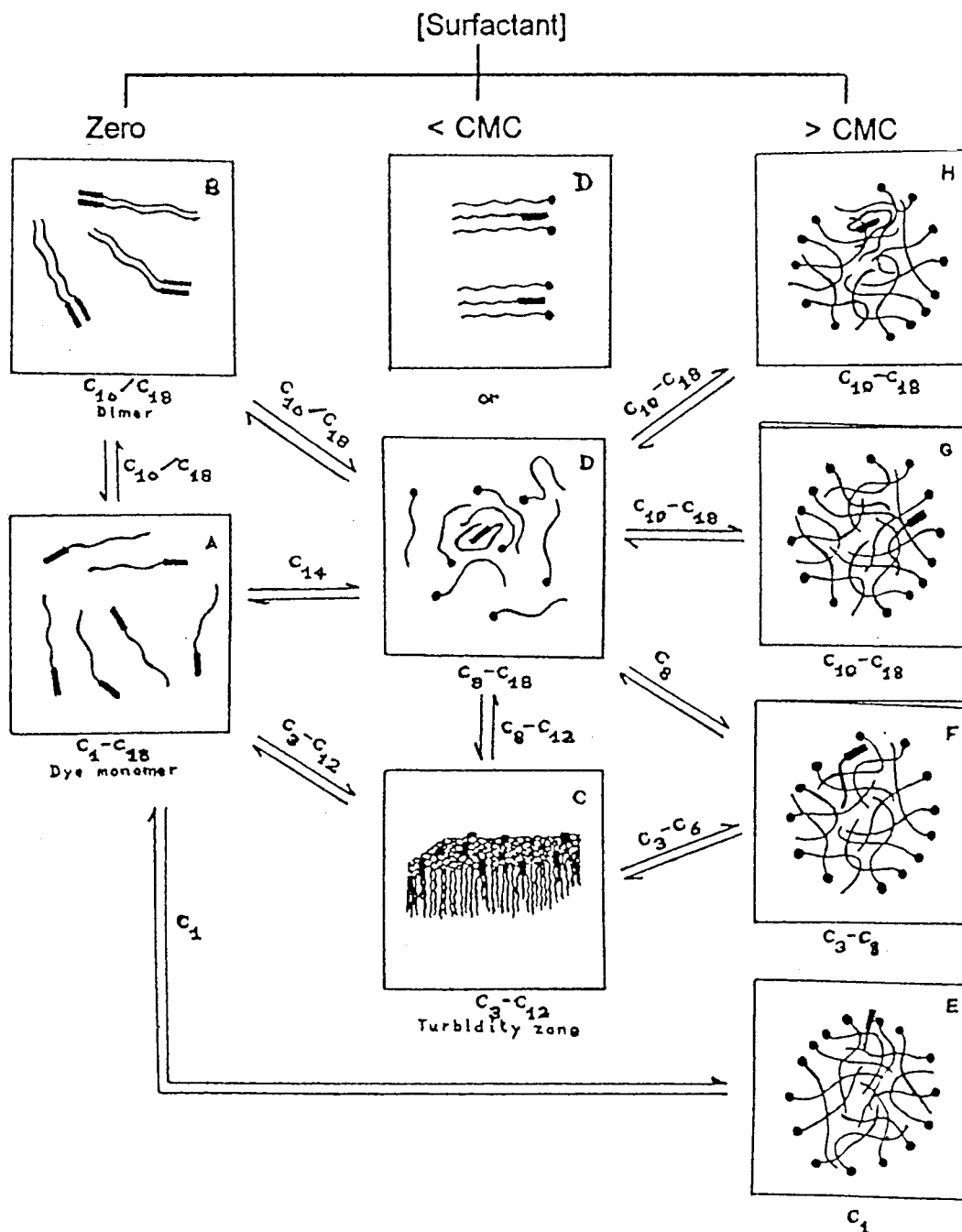
Figure 15. Structural hierarchy of the dyes ( 86 : C 1 –C 18 ) in 2% MeOH with varying concentration of SDS. Cationic dye molecules with varying chain length: ■~. Surfactant molecules (SDS): •~. (A) C 1 –C 18 dye monomers in 2% MeOH. (B) C 10 –C 18 dimers in 2% MeOH. (C) Probable structure of the turbidity of C 3 –C 12 dyes and SDS (<CMC). (D) Coiling of C 8 –C 18 dyes below the CMC of SDS. (E–H) Localization of the chromophoric headgroup at various distances from the micellar interface. (Reprinted with permission from ref 345. Copyright 1999 Elsevier Science.)
